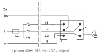
3 circuit DALI track system
