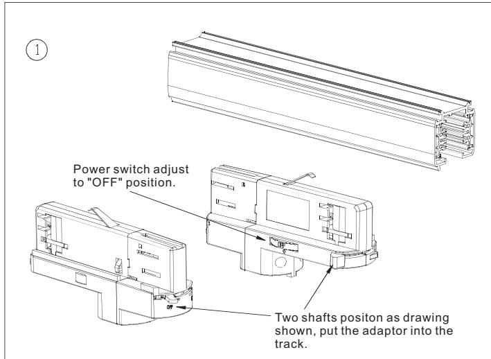
ADAPTOR INSTALLATION DIAGRAM
