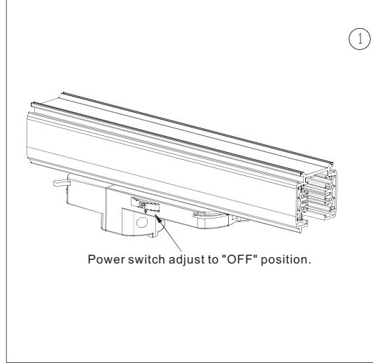
ADAPTOR DISASSEMBLY DIAGRAM
